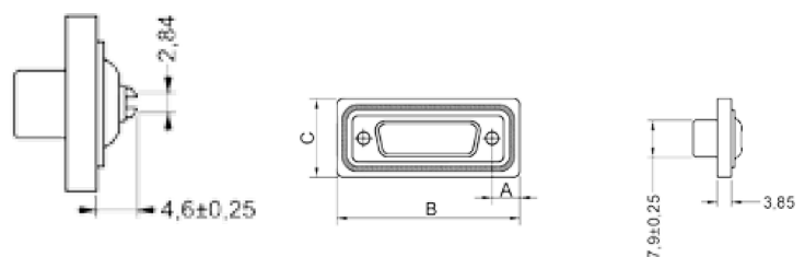
Standard D-Sub Connectors: Solder
